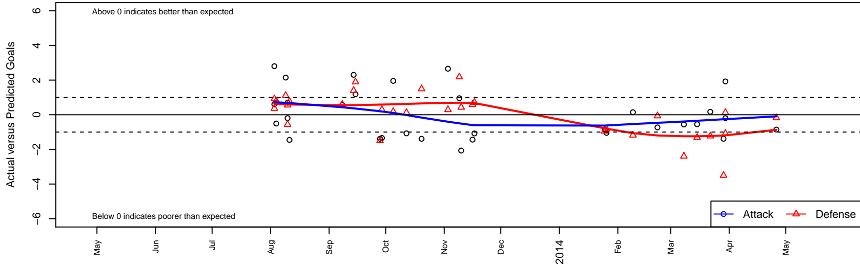
SSC Shadow B G01 Dots are actual minus expected GF (blue circles) and GA (red triangles). Blue line is smoothed change in attack strength. Red is smoothed change in defense strength.
